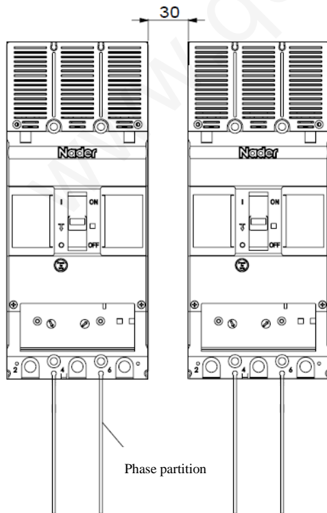
Safety Mounting Spacing between Circuit Breakers
